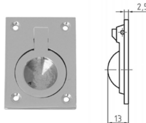
Flush pull #46.108 chrome plated: 52 x 37 mm
