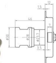
latch #21.711Z; 30 mm backset, brass chrome plated
