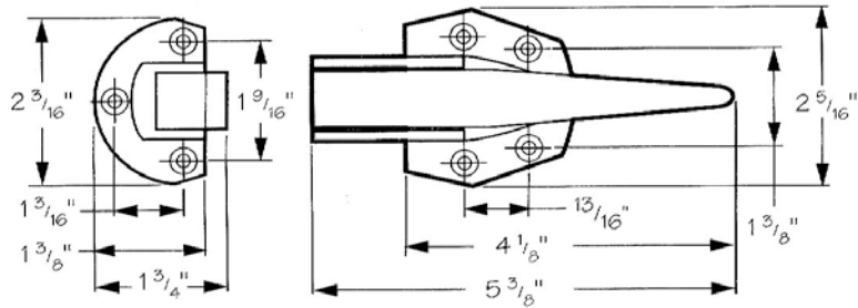
#88.066 Latch for up lay doors with 1/2 inch offset; stainless steel , with padlock provision Base 2 5/16 inch x 2 3/16 inch" Strike sold separate #88.067 Strike for offset adjustable 5/8 x 1 1/4 inch
