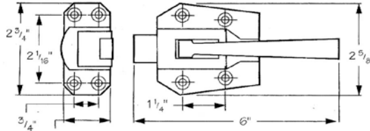
88.163 Latch for up lay doors with 1/2 inch offset; stainless steel , with padlock provision Base 2 5/8" x 3" Strike included
